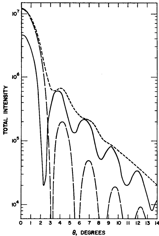
FIGURE 1 Total (both polarizations) Mie scattering intensity (—) as a function of the scattering angle, \theta , for \alpha = 70 , m = 1.05 . The Hodkinson model (----) and diffraction (— · —) results are shown for comparison.
