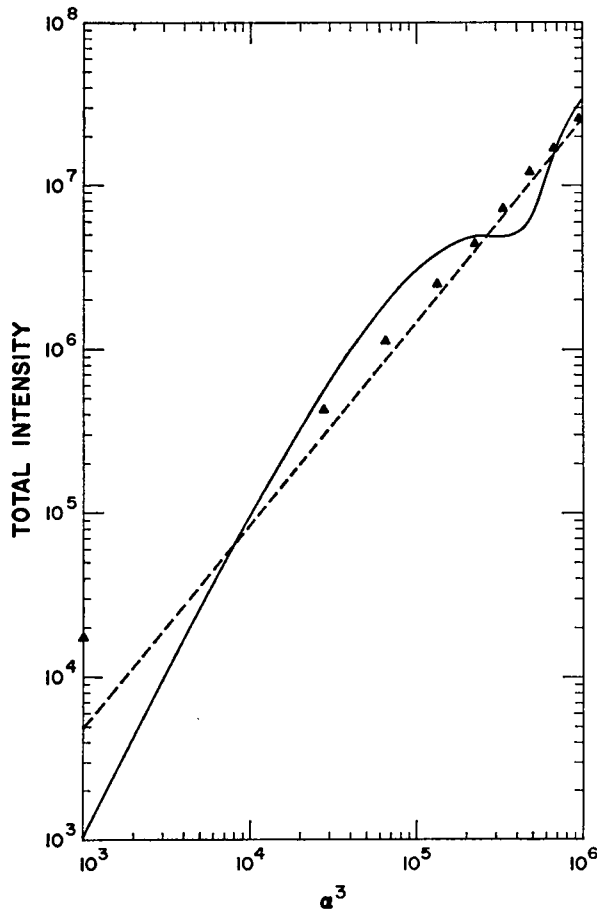
FIGURE 3 Total scattering intensity at \theta = 0.5^\circ calculated with the codes DAMIE and DBMIE for m = 1.05 as a function of \alpha^3 (—). Also shown are the equivalent Hodgkinson result ( \blacktriangle ) and diffraction result (-----).
